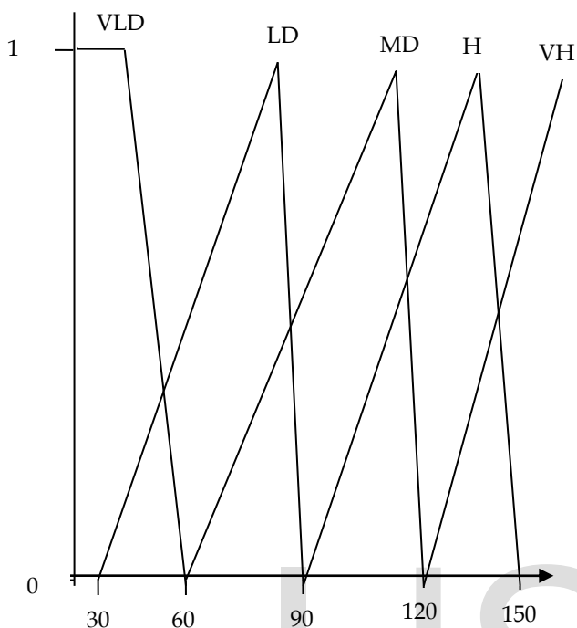
Fig. 2. Triangular membership function for traffic density fuzzifier In fuzzy inference process, it is important to establish a system, which indicates how to project input variables onto output space. This can be achieved by specifying if-then fuzzy rules. A single fuzzy if-then rule follows the form:
